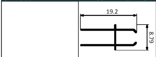
GM-79831 SCREEN ASTRAGAL
