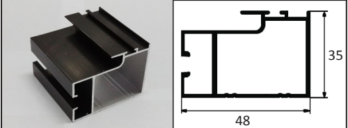
GM-99910 FIXED HEAD
