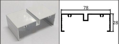
GM-99914 PANEL ASTRAGAL
