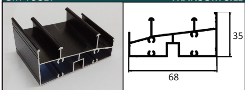
GM-79825 TRANSOM GLASS DIVIDER
