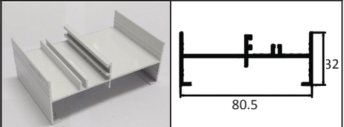
GM-99905 OUTER BOTTOM RAIL
