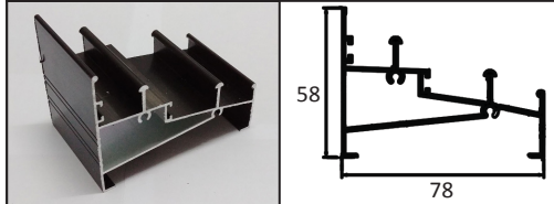
GM-99904 TOP RAIL
