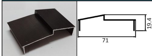
GM-79814 PANEL ASTRAGAL
