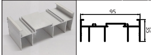
OS-97803 DOUBLE JAMB (3 Tracks)
