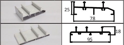
DOUBLE FLAT SILL/DOUBLE FLAT SILL 3 Tracks
