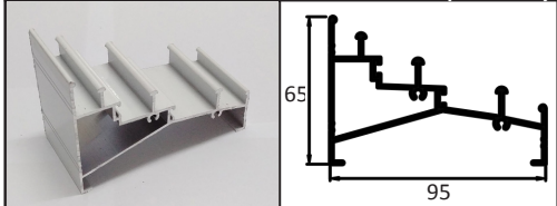
GM-99901 DOUBLE HEAD
