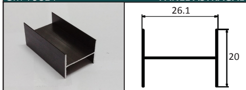
GM-79819 DOUBLE FLAT SILL
