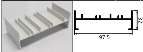
GM-99902 DOUBLE SILL
