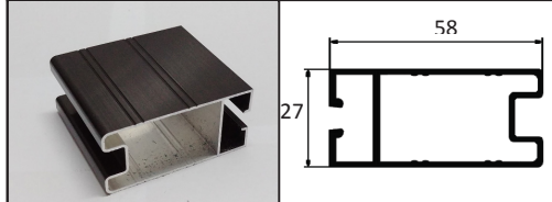
GM-99904A INNER BOTTOM RAIL
